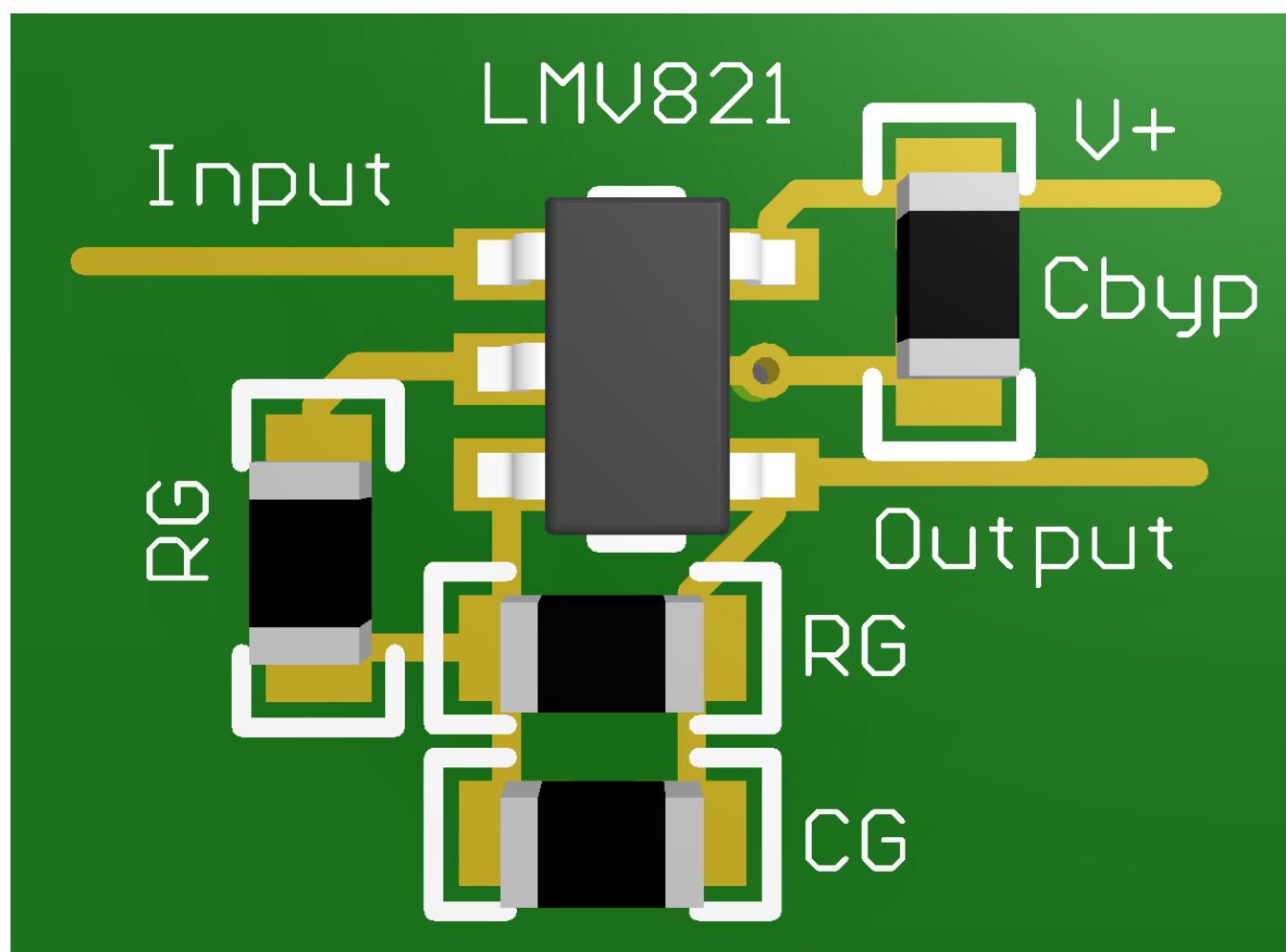
Figure 48. 3-D Layout
